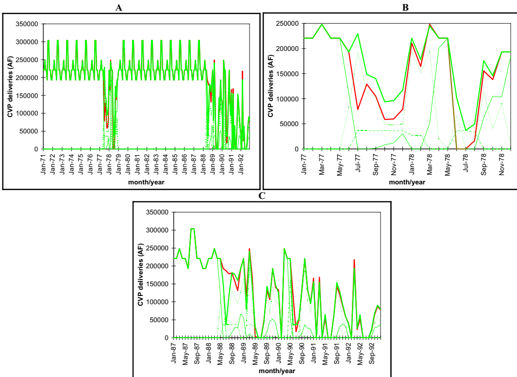
Figure 30: Deliveries to the CVP Demand Node for the Base Case (red) and Isolated Facility/1.2 MAF Conjointive Use Alternative (green) A: Over the Entire Simulated Time Horizon; B: During the 1977-1978 Drought; and C: During the 1987-1992 Drought (heavy solid line: total deliveries; light solid line: Delta pumping; short dashed line: Isolated Facility; long dashed line: aquifer storage)
