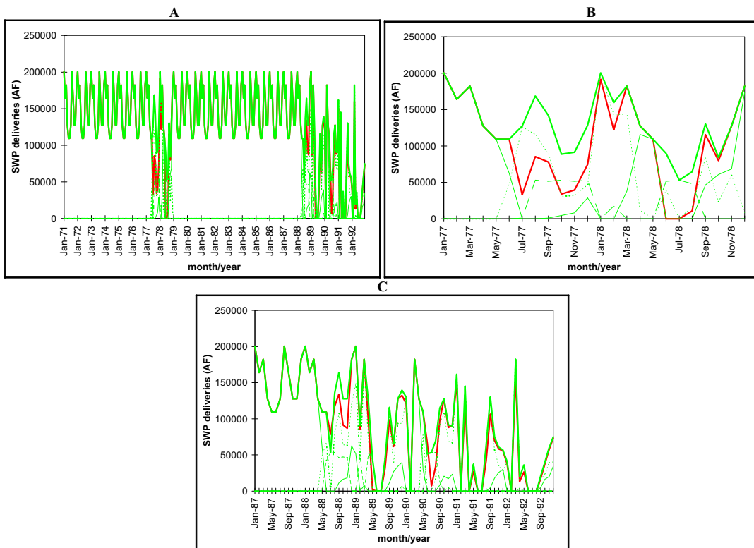
Figure 29: Deliveries to the SWP Demand Node for the Base Case (red) and Isolated Facility/1.2 MAF Conjointive Use Alternative (green) A: Over the Entire Simulated Time Horizon; B: During the 1977-1978 Drought; and C: During the 1987-1992 Drought (heavy solid line: total deliveries; light solid line: Delta pumping; short dashed line: Isolated Facility; long dashed line: aquifer storage)
